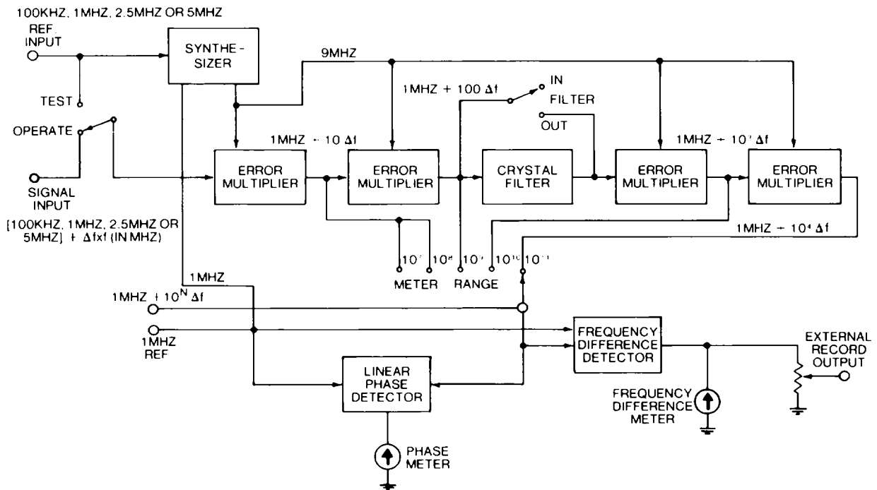
Block Diagram of the Model 527E Frequency Difference Meter
